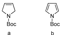
Figure 2. Structures of (a) N -( tert -butoxycarbonyl)-3-pyrroline and (b) N -( tert -butoxycarbonyl)pyrrole.
