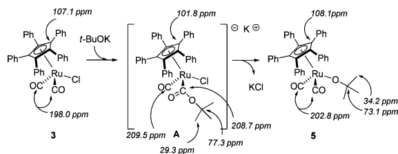
Scheme 2. Detection of Acyl Intermediate A by ^{13}\text{C} NMR in Toluene- d_8 at -32\text{ }^{\circ}\text{C}
