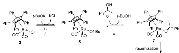
Scheme 1. Proposed Mechanism of Racemization of sec -Alcohols by Ruthenium Catalyst 3
