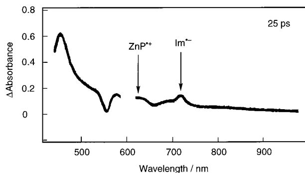
Figure 3. Differential absorption spectra obtained upon picosecond flash photolysis (590 nm) of \sim 10^{-4} M solutions of ZnP-Im-CH 2 -ref in argon saturated THF with a time delay of 25 ps.
