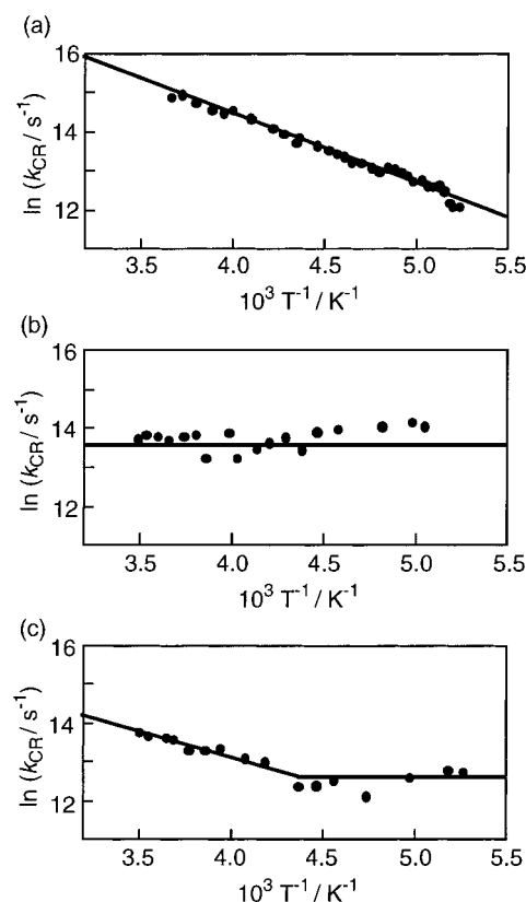
Figure 7. Arrhenius plots of k_{\text{CR}} for the intramolecular CR process from C 60 •- to ZnP •+ in (a) ZnP-Im-CH 2 -C 60 , (b) ZnP-Im-C 60 , and (c) ZnP-CH 2 -Im-C 60 in THF.
