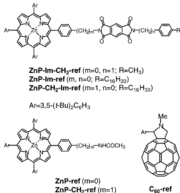
Figure 2. Porphyrin-pyromellitimide dyads and porphyrin and C 60 references.
