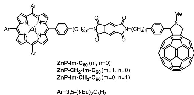
Figure 1. Porphyrin-pyromellitimide-C 60 triads.
