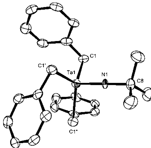
Figure 1. ORTEP diagram of the X-ray crystal structure of 1 . Ta–C 1 = Ta–C 1' = Ta–C 1'' = 2.216 Å. Ta–N 1 = 1.737 Å. Ta–N 1 –C 8 = 180.0°.
