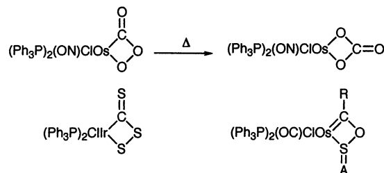
Scheme 8. Perchalcometallacycles a
