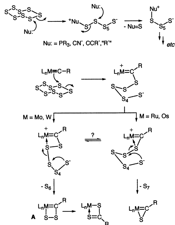
Scheme 8. Perchalcometallacycles a
