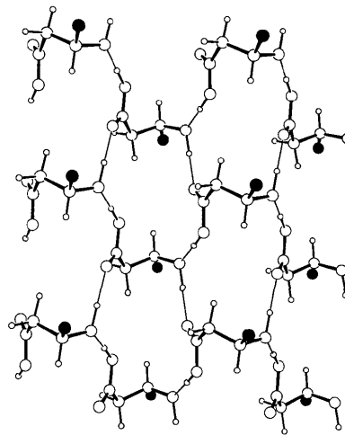
Fig. 4. Schematic drawing (Johnson, 1976) illustrating the sheet-like O—H...O hydrogen bonding network for 3-hydroxy-3-phenylpropionic acid. The phenyl group is replaced by C4 (drawn black) for clarity. All atoms are drawn as spheres with a fixed radius. The O—H...O hydrogen bonds are shown as thin lines.
