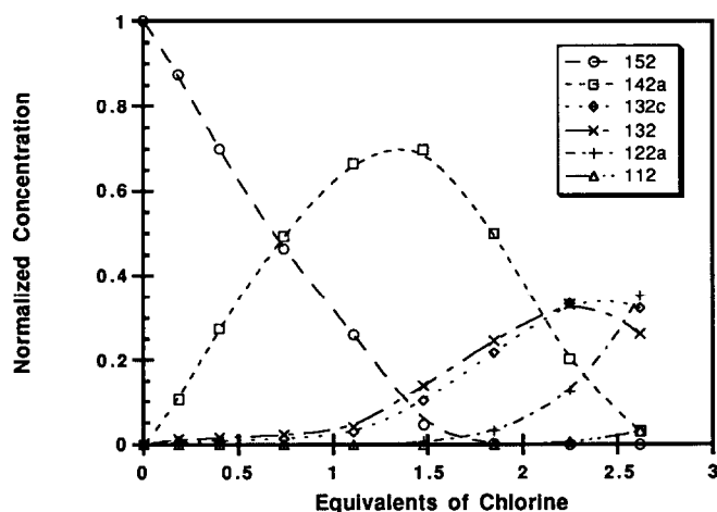
Fig. 1. The photochlorination of \text{CH}_2\text{FCH}_2\text{F} in \text{CCl}_4 .
