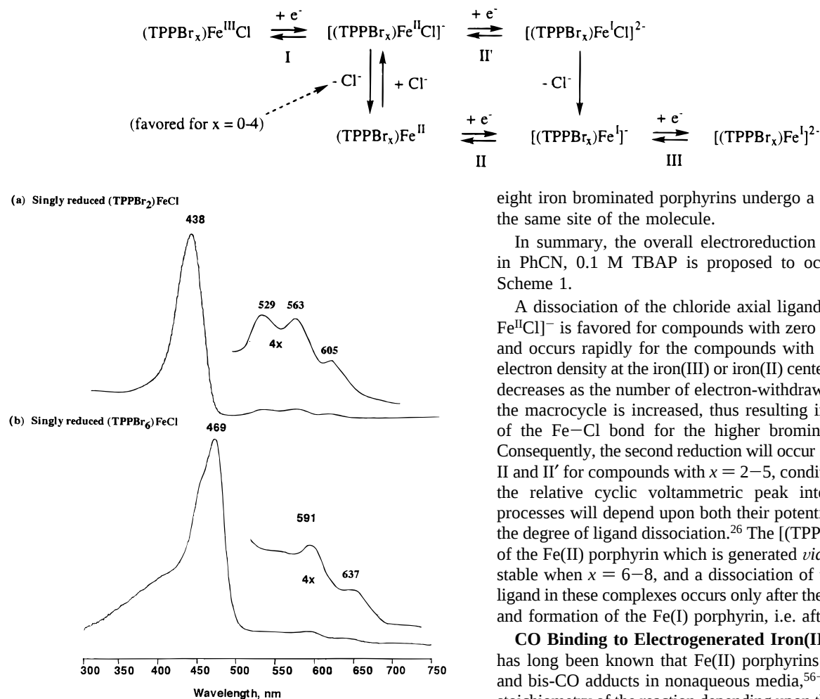
Figure 5. Electronic absorption spectra of singly reduced (a) (TPPBr 2 )FeCl and (b) (TPPBr 6 )FeCl in PhCN, 0.2 M TBAP.
