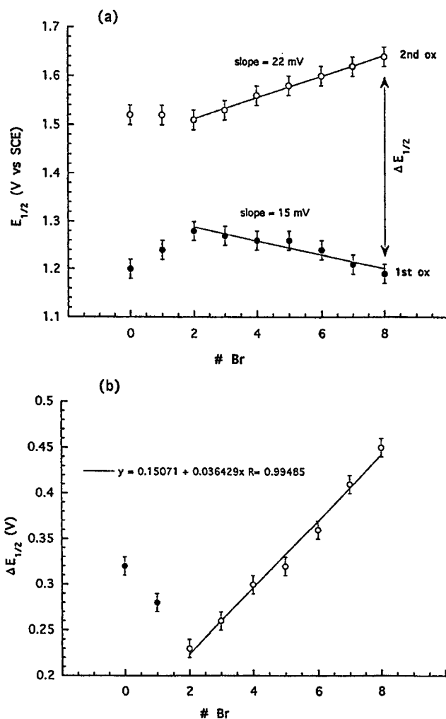
Figure 3. Plots of (a) E_{1/2} vs the number of Br groups for the first and second oxidations of (TPPBr x )FeCl and (b) \Delta E_{1/2} between the first and second oxidations of (TPPBr x )FeCl vs the number of Br groups.
