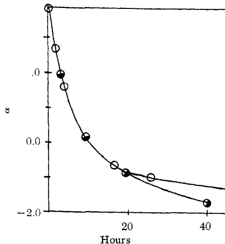
Fig. 1.—The optical rotation-time curve for the alcoholysis of d - \alpha -PhCHClMe in EtOH with added \text{HgCl}_2 (data of Table III). O represents the experimental curve; — the theoretical curve calculated by equation (23), example 3.
