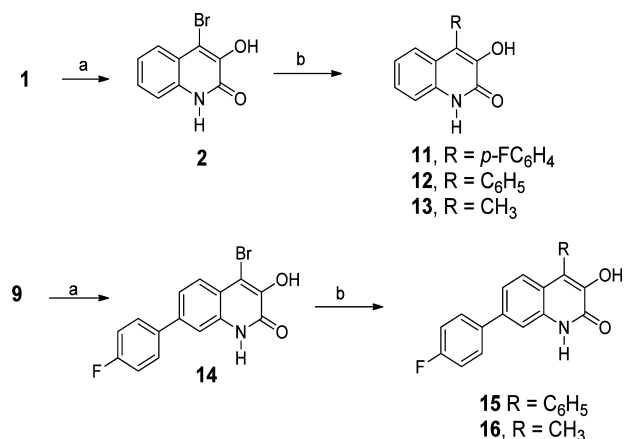
Scheme 2. Formation of Compounds 2 and 14 and Use in Suzuki-Coupling Reactions a
