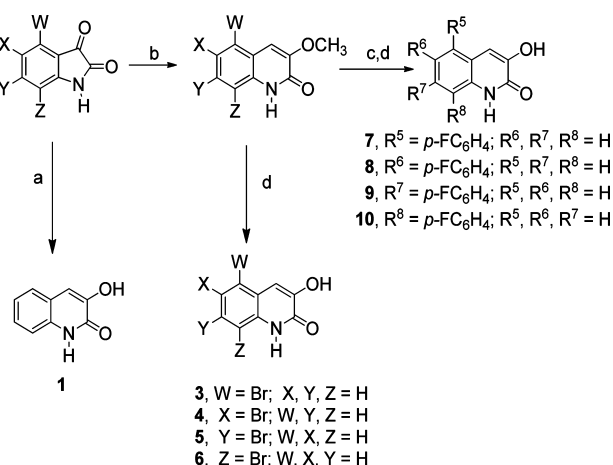
Scheme 1. Synthesis of 3-Hydroxyquinolin-2(1H)-one, 5-, 6-, 7-, and 8-Bromo 3-Hydroxyquinolin-2(1H)-ones, and 5-, 6-, 7-, and 8-( p -Fluorophenyl) 3-Hydroxyquinolin-2(1H)-ones a
