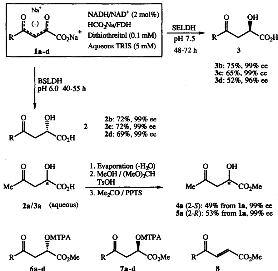
Scheme 1 a: R = Me; b: R = i -Pr; c: R = n -C 6 H 13 ; d: R = Ph
