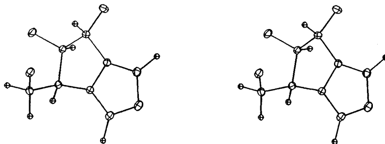
Figure. Stereopair view of 8 . Hydroxy H-atoms are not represented.
