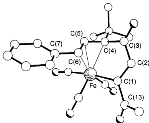
Fig. 1 Molecular structure of complex 11 ( R^1 = \text{MeCO} , R^2 = \text{H} , R^3 = \text{Bu}^t ) ( \text{C}_{21}\text{H}_{20}\text{FeO}_5 ). Selected bond lengths ( \text{\AA} ) and bond angles ( ^\circ ): C(1)–C(2) 1.350(13), C(2)–C(3) 1.441(13), C(3)–C(4) 1.552(13), C(4)–C(5) 1.412(11), C(5)–C(6) 1.404(12), Fe–C(1) 2.017(10), Fe–C(4) 2.205(8), Fe–C(5) 2.079(8), Fe–C(6) 2.182; Fe–C(1)–C(13) 122.2(7), Fe–C(1)–C(2) 117.2(7), C(1)–C(2)–C(3) 118.5(9), C(2)–C(3)–C(4) 115.3(8), C(3)–C(4)–C(5) 114.0(8), C(4)–C(5)–C(6) 123.3(8), C(5)–C(6)–C(7) 123.8(8).
