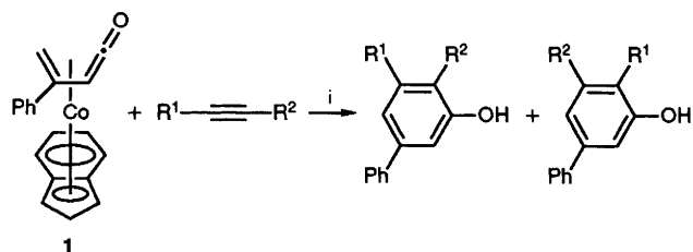
Scheme 1 Reagents and conditions: i, cycloocta-1,5-diene (2 equiv.), 100 °C, 19–21.5 h, (45–92%)
