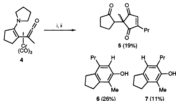
Scheme 3 Reagents and conditions: i, pent-1-yne, tetrahydrofuran, 85 °C, 2–4 h; ii, SiO 2 or TiCl 3 –LiAlH 4
