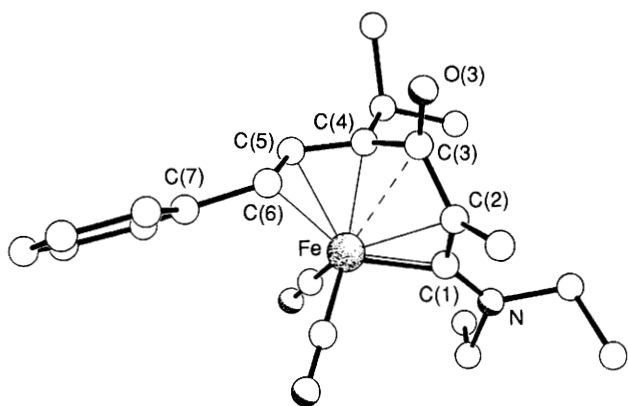
Fig. 2 Molecular structure of one of the pair of crystallographically independent molecules of 12 ( R^1 = \text{Et}_2\text{N} , R^2 = \text{Me} , R^3 = \text{Pr}^i ) [ 2(\text{C}_{22}\text{H}_{27}\text{FeNO}_8 \cdot \text{H}_2\text{O}) ]. Selected bond lengths ( \text{\AA} ) and bond angles ( ^\circ ) (values in [ ] refer to the second independent molecule): C(1)–C(2) 1.408(7) [1.424(6)], C(2)–C(3) 1.430(7) [1.430(9)], C(3)–C(4) 1.507(8) [1.513(7)], C(4)–C(5) 1.416(9) [1.417(8)], C(5)–C(6) 1.398(5) [1.355(7)], Fe–C(1) 1.833(6) [1.841(7)], Fe–C(2) 2.184 [2.187(5)], Fe–C(3) 2.436(6) [2.436(5)], Fe–C(4) 2.073(5) [2.061(5)], Fe–C(5) 2.080(5) [2.072(7)], Fe–C(6) 2.174(5) [2.156(6)], C(1)–N 1.301(7) [1.297(8)], C(3)–O(3) 1.235(6) [1.241(6)], Fe–C(1)–N 145.1(5) [146.1(4)], Fe–C(1)–C(2) 83.6(4) [83.0(4)], C(1)–C(2)–C(3) 118.0(4) [117.8(5)], C(2)–C(3)–C(4) 111.8(5) [111.9(4)], C(3)–C(4)–C(5) 114.6(4) [113.1(4)], C(4)–C(5)–C(6) 121.9(5) [123.7(5)], C(5)–C(6)–C(7) 122.6(5) [124.1(5)].
