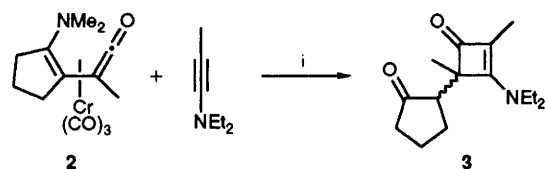
Scheme 2 Reagents and conditions: i, benzene, 25 °C, 18 h, (36%)
