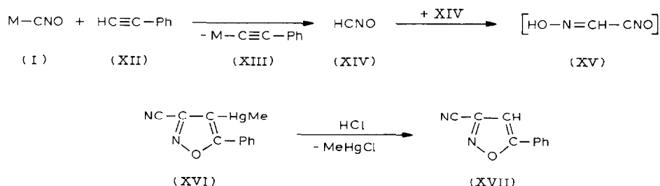
SCHEME 3. a, M = Me 3 Si; b, M = MeHg.
