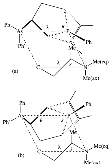
Figure 2. Interchelate interactions (a) in (+)- 3 and (b) in the unfavored diastereomer.
