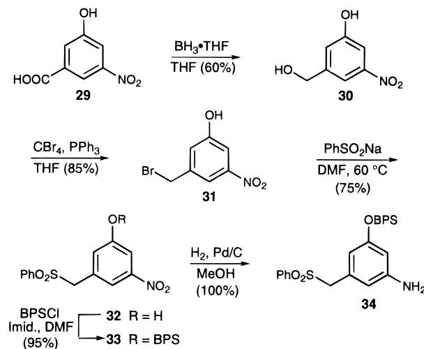
Scheme 6
