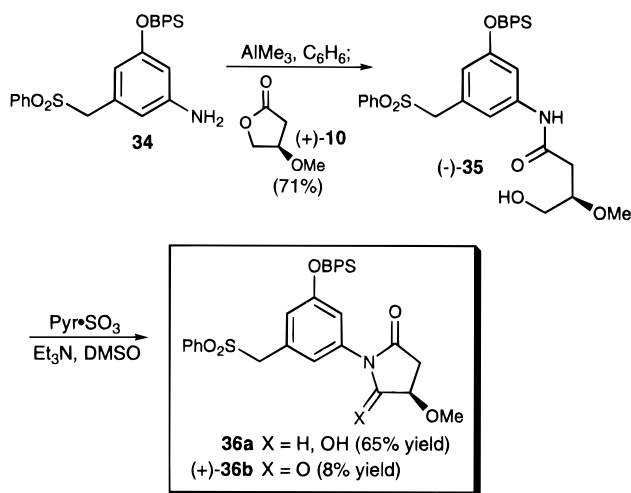
Scheme 7
