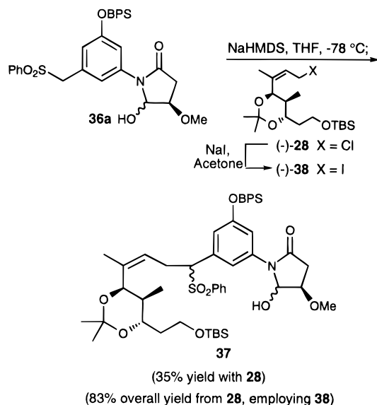
Scheme 8
