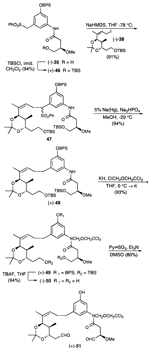
Scheme 11
