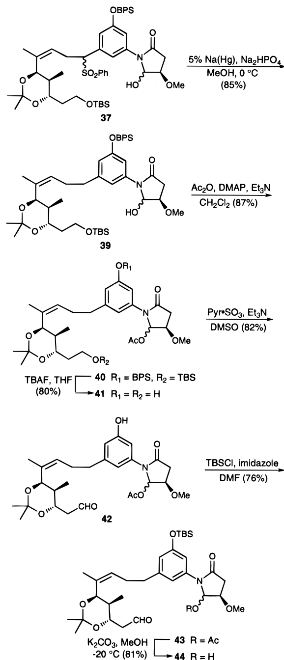
Scheme 9
