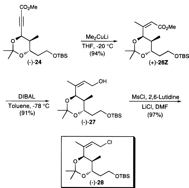
Scheme 5
