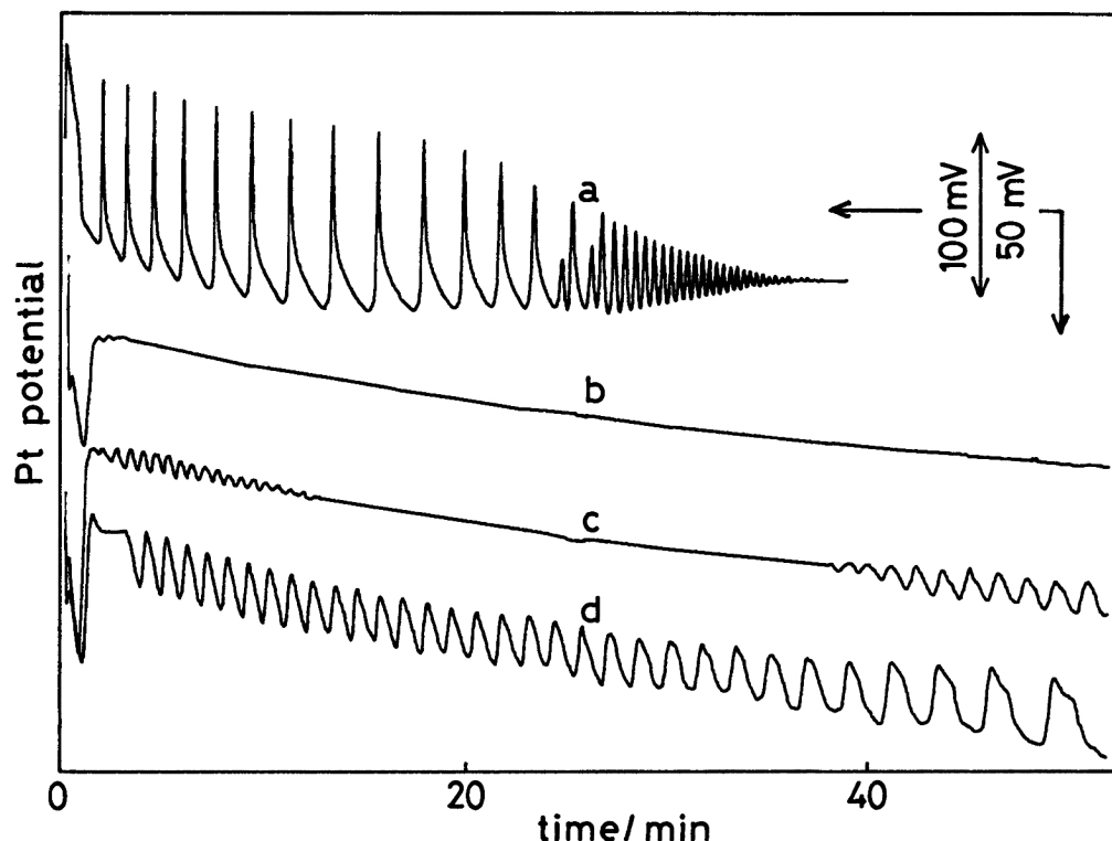
Fig. 3. Potential-time profiles. MA system (a): 2.01 M MA, 0.048 M \text{Ce}(\text{NO}_3)_3 , and 0.451 M \text{KBrO}_3 at 30 °C. AA system: 0.020 M(b), 0.019 M(c), and 0.018 M(d) AA. Other components are in standard conditions.
