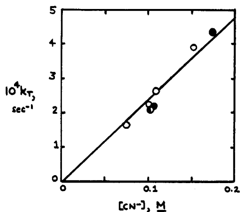
Figure 1. First-order rate constants for cyanide-catalyzed detritiation of C_6H_5CTO , as a function of cyanide concentration, in CH_3OH (open circles), CH_3OD (filled circles), and 50% CH_3OH -50% CH_3OD (half-filled circle).
