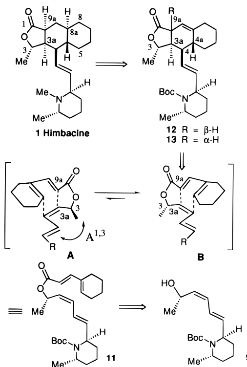
Scheme 1
