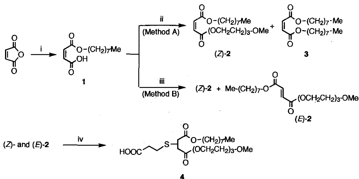
Scheme 1 Reagents and conditions : i) HO-(CH 2 ) 7 -Me in dry benzene, reflux ; ii) H-(OCH 2 CH 2 ) 3 -OMe / p -TsOH in dry benzene, reflux ; iii) H-(OCH 2 CH 2 ) 3 -OMe / DCC / DMAP in CH 2 Cl 2 , room temperature; iv) HSCH 2 CH 2 COOH / NaOH / piperidine in 2-propanol, reflux.
