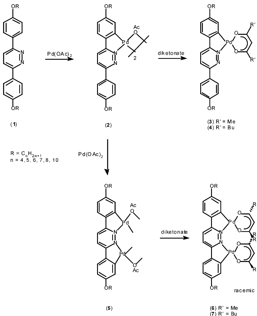
Scheme 1.
