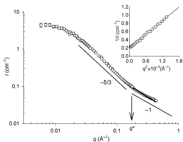
Figure 1. Scattered intensity as a function of q at T = 20^\circ\text{C} ( \circ ) for a solution of dynamer (1,8) formed in deuterated acetone from 1 and 8 at an initial concentration of 100 mM (thick black line: des Cloizeaux fit). The inset graph represents the variation of 1/I as a function of q^2 .
