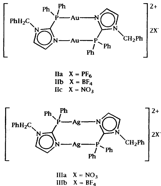
Fig. 1. Scheme of the compounds studied.
