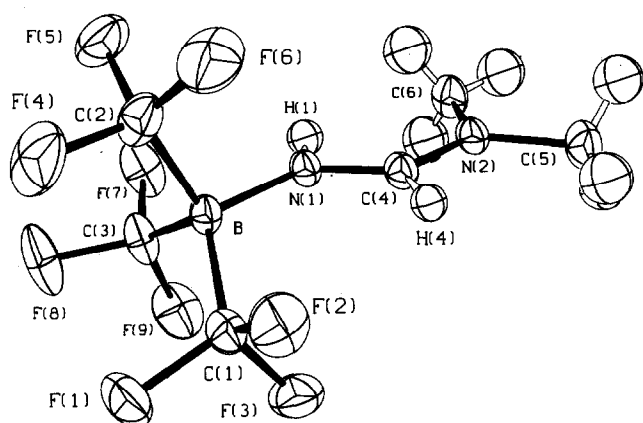
Fig. 3. Perspective drawing of (\text{CF}_3)_3\text{B} \cdot \text{NH}=\text{CHNMe}_2 .
