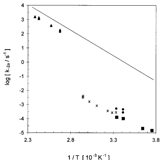
Figure 3. Thermal decay rate constants of \text{BrNO}_2 ( \text{BrONO} ): triangles, from ref 3, p = 267 \text{ mbar} , \text{M} = \text{N}_2 , isomer assumed to be \text{BrNO}_2 ; straight line, calculated from ref 3 for p = 1 \text{ bar} ; crosses, ref 4, isomer \text{BrNO}_2 , p = 1000 \text{ mbar} , \text{M} = \text{He} , propene added in order to scavenge \text{Br} atoms; full squares, this work, isomer \text{BrNO}_2 , p = 988 \pm 2 \text{ mbar} , \text{M} = \text{synthetic air} , trans -2-butene added in order to scavenge \text{Br} atoms; full circles, 293/300 K, 805 \pm 5 \text{ mbar} , \text{M} = \text{synthetic air} , [\text{Br}_2]_0 = 7.8 \times 10^{14} \text{ molecule cm}^{-3} , [\text{NO}_2]_0 = 1.6 \times 10^{14} \text{ molecule cm}^{-3} , excess \text{CH}_3\text{CHO} ( 3.5 \times 10^{15} \text{ molecule cm}^{-3} ) added in order to scavenge \text{Br} atoms.
