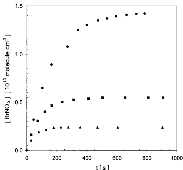
Figure 1. Concentration–time profiles for \text{BrNO}_2 formation at different initial concentrations of \text{NO}_2 , T = 293 \pm 1 \text{ K} , p = 988 \pm 2 \text{ mbar} , M = \text{N}_2 ; initial concentrations (in molecule \text{cm}^{-3} ): triangles, [\text{Br}_2]_0 = 7.1 \times 10^{14} , [\text{NO}_2]_0 = 1.7 \times 10^{14} ; squares, [\text{Br}_2]_0 = 7.1 \times 10^{14} , [\text{NO}_2]_0 = 3.5 \times 10^{14} ; circles, [\text{Br}_2]_0 = 8.2 \times 10^{14} , [\text{NO}_2]_0 = 7.1 \times 10^{14} .
