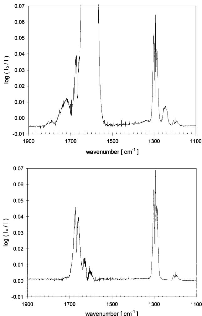
Figure 2. IR spectra during photolysis of a \text{Br}_2/\text{NO}_2/\text{N}_2 mixture with 500–700 nm light, photolysis time, 475 s, T = 292 \text{ K} , p = 989 \text{ mbar} , M = \text{N}_2 , [\text{Br}_2]_0 = 8.2 \times 10^{14} \text{ molecule cm}^{-3} , [\text{NO}_2]_0 = 7.1 \times 10^{14} \text{ molecule cm}^{-3} , water vapor absorption lines have been subtracted from both spectra: (a, top) product spectrum; (b, bottom) absorptions from \text{NO}_2 , \text{N}_2\text{O}_5 , and traces of \text{BrNO} subtracted from spectrum a, showing the IR absorptions of \text{BrNO}_2 centered at 1200, 1292, and 1667 \text{ cm}^{-1} ; between 1580 and 1640 \text{ cm}^{-1} there is residual absorption from the nearly saturated \text{NO}_2 band.
