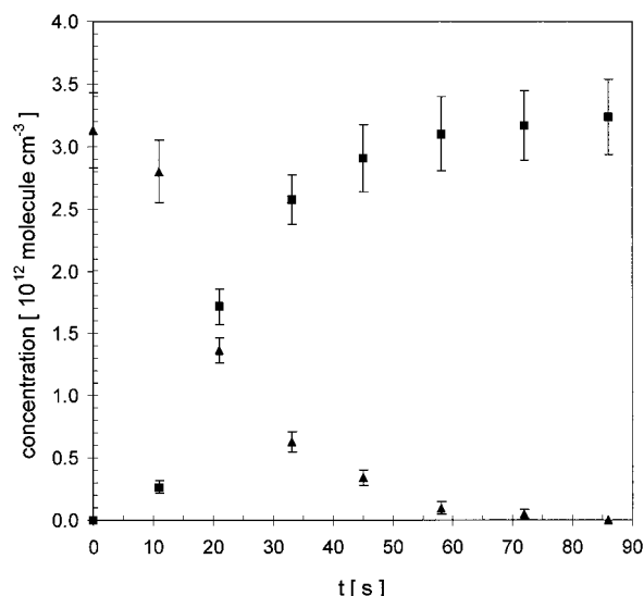
Figure 6. Concentration–time profiles of \text{BrNO}_2 (triangles) and \text{BrNO} (squares) in the dark; reaction conditions same as in Figure 5. During the initial 10 s, the time behavior deviates from first order owing to the finite mixing time of the added NO. In Figure 4, the time of the second data point of each profile is set equal to zero.
