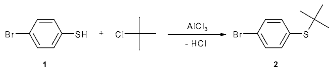
SCHEME 1 Synthesis of (4-bromo)phenyl- tert -butylthioether 2 .
