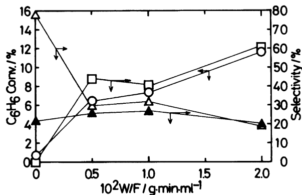
Fig. 4. The effect of W/F on the oxidative coupling of benzene on \text{Sm}_2\text{O}_3 at 873 K. Reaction conditions: same as Fig. 2 except the weight of catalyst ( W ). W = 0 g at W/F = 0 , W = 0.15 g at W/F = 0.5 \times 10^{-2} , W = 0.3 g at W/F = 1.0 \times 10^{-2} and W = 0.6 g at W/F = 2.0 \times 10^{-2} . Symbols: same as Fig. 3.
