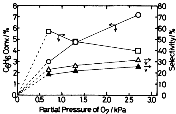
Fig. 3. The effect of partial pressure of oxygen on the oxidative coupling of benzene on \text{Sm}_2\text{O}_3 at 873 K. Reaction conditions: same as Fig. 2 except the partial pressure of \text{O}_2 . Symbols: \circ \text{C}_6\text{H}_6 conversion, \square \text{C}_{12}\text{H}_{10} selectivity, \triangle \text{CO}_2 selectivity, \blacktriangle CO selectivity.
