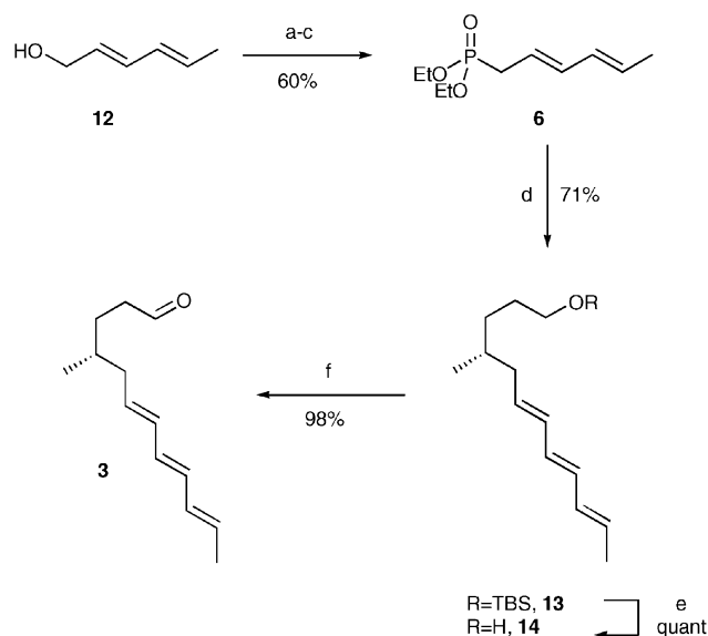
Scheme 3 Reagents and conditions: (a) \text{BuLi} , THF, -10^\circ\text{C} ; (b) \text{TsCl} , -10^\circ\text{C} ; (c) (\text{EtO})_2\text{PNa} , -78^\circ\text{C} to rt; (d) \text{BuLi} , THF, -78^\circ\text{C} , then 11 , -78^\circ\text{C} to rt; (e) \text{TBAF} , THF, 0^\circ\text{C} to rt; (f) \text{DMSO} , (\text{COCl})_2 , \text{Et}_3\text{N} , \text{CH}_2\text{Cl}_2 , -78^\circ\text{C} to rt.
