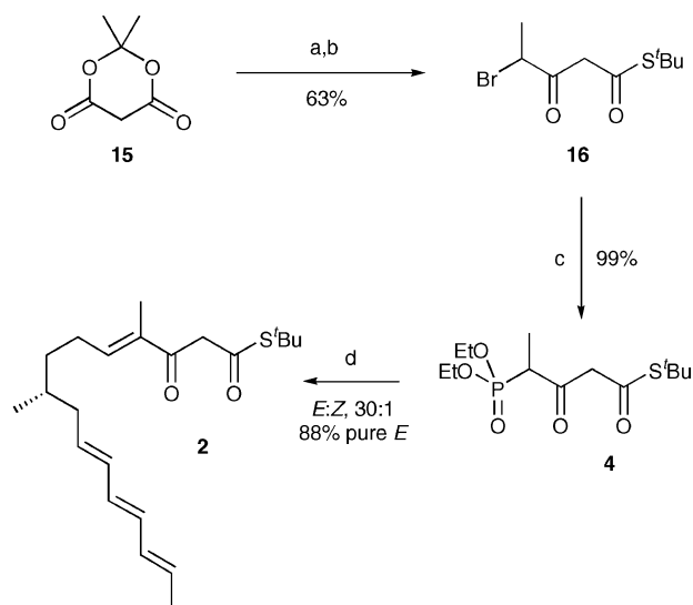
Scheme 4 Reagents and conditions: (a) \text{CH}_3\text{CHBrCOBr} , pyridine, \text{CH}_2\text{Cl}_2 , 0^\circ\text{C} ; (b) \text{BuSH} , \text{PhH} , reflux; (c) \text{NaH} , THF, -30^\circ\text{C} to -20^\circ\text{C} , then (\text{EtO})_2\text{PNa} , THF, -20^\circ\text{C} to rt; (d) \text{KHMDs} , THF, -78^\circ\text{C} , then 3 .
