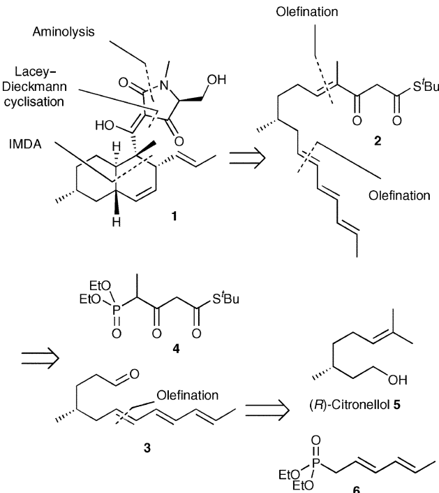
Scheme 1 Retrosynthetic analysis.
