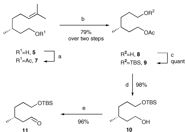
Scheme 2 Reagents and conditions: (a) \text{Ac}_2\text{O} , pyridine, \text{CH}_2\text{Cl}_2 ; (b) \text{O}_3 , \text{CH}_2\text{Cl}_2 , -78^\circ\text{C} then \text{MeOH} , \text{NaBH}_4 , 0^\circ\text{C} ; (c) \text{TBSCl} , imidazole, THF, rt; (d) \text{MeOH} , \text{K}_2\text{CO}_3 cat., rt; (e) \text{DMSO} , (\text{COCl})_2 , \text{Et}_3\text{N} , \text{CH}_2\text{Cl}_2 , -78^\circ\text{C} to rt.
