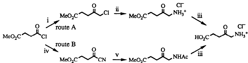
Scheme 3. Reagents: i, CH 2 N 2 then HCl; ii, NaN 3 then H 2 /Pd; iii, HCl; iv, CuCN; v, Zn/AcOH/Ac 2 O.
