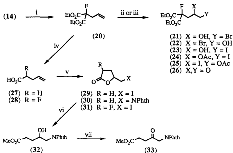
Scheme 6. Reagents: i, NaH/allyl bromide/DMF; ii, NBS/DMSO/H 2 O; iii, AgOAc/I 2 ; iv, NaCl/DMSO/H 2 O then KOH; v, I 2 /NaHCO 3 then PhthNK/DMF; vi, KOH then CH 2 N 2 ; vii, CrO 3 /H 2 SO 4 .
