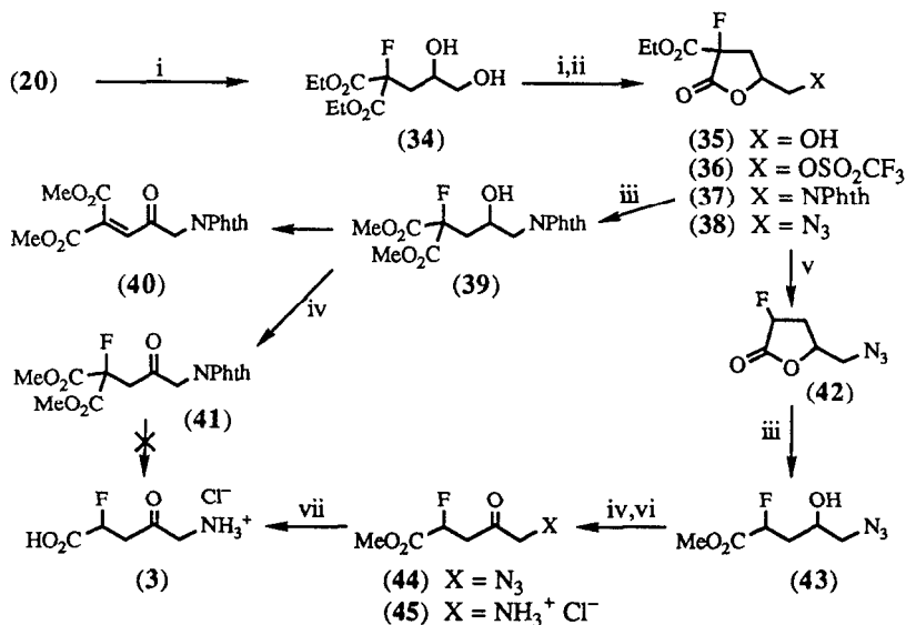
Scheme 7. Reagents: i, \text{OsO}_4/\text{NMO} ; ii, \text{Tf}_2\text{O}/\text{Pyr} then PhthNK or \text{NaN}_3 ; iii, KOH then \text{CH}_2\text{N}_2 ; iv, \text{CrO}_3/\text{H}_2\text{SO}_4 ; v, \text{NaCl}/\text{DMSO}/\text{H}_2\text{O} ; vi, \text{H}_2/\text{Pd} ; vii, aq. HCl.
