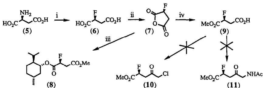
Scheme 4. Reagents: i, \text{NaNO}_2/\text{HF}/\text{Py} ; ii, TFAA; iii, menthol/DMAP then \text{CH}_2\text{N}_2 ; iv, MeOH.
