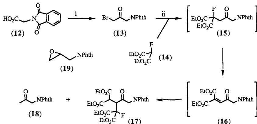
Scheme 5. Reagents: i, \text{ClCO}_2\text{Et}/\text{Et}_3\text{N} then \text{CH}_2\text{N}_2 then \text{HBr} ; ii, (14)/ \text{NaH}/\text{DMF} .
