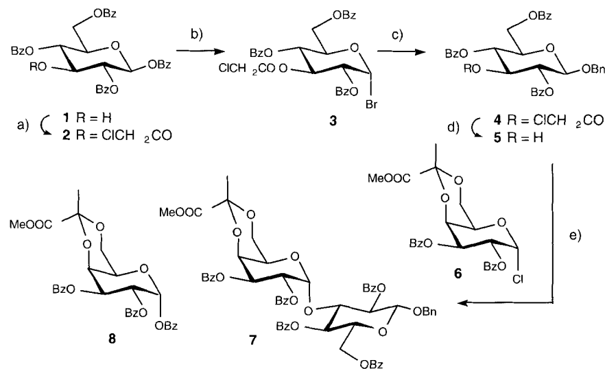
Scheme 2 a) 1 [14] (1 eq.), (\text{ClCH}_2\text{CO})_2\text{O} (6.2 eq.), \text{NaHCO}_3 (1.2 eq.), DMF, 2 h, 25 °C, 87%; b) 2 (1 eq.), HBr (30% in AcOH), \text{CH}_2\text{Cl}_2 , 1.5 h, 25 °C, 93%; c) benzyl alcohol (1 eq.), AgOTf (1.25 eq.), 3 (0.74 eq.), 2,4,6-trimethylpyridine (0.67 eq.), \text{CH}_2\text{Cl}_2 , 10 min., 25 °C, 69%; d) 4 (1 eq.), thiourea (2 eq.), MeOH, 14 h, 25 °C, 6 h, 60 °C, 100%; e) 1) 5 (1 eq.), AgOTf (1.5 eq.), 6 [16] (0.88 eq.), 2,4,6-trimethylpyridine (0.7 eq.), \text{CH}_2\text{Cl}_2 , 0.5 h, 25 °C; 2) pyridine/benzoyl chloride (2:1), 0.5 h, 25 °C, 69% 7 , 22% 8 .
