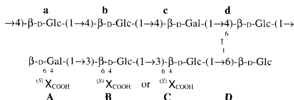
Scheme 1 Repeating unit of the exopolysaccharide of Rhizobium leguminosarum biovar phaseoli (CIAT 899) [7].
