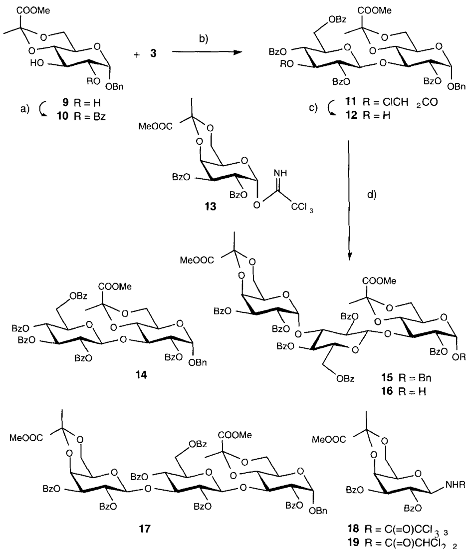
Scheme 3 a) [13]; b) 10 (1 eq.), AgOTf (1.5 eq.), 3 (1.2 eq.), 2,4,6-trimethylpyridine (0.8 eq.), CH_2Cl_2 , 35 min., 25 °C, 85%; c) 11 (1 eq.), thiourea (2 eq.), CH_2Cl_2/MeOH , 19 h, 60 °C, 100%; d) 1) 12 (1 eq.), TMSOTf (0.1 eq.), 13 (1.1 eq.), CH_2Cl_2 , 0.5 h, 0 °C; 2) pyridine/benzoyl chloride (2:1), 1 h, 25 °C, 44% 14 , 26% 15 , 26% crude 17 ; 3) 12 (1 eq.), TMSOTf (0.1 eq.), 13 (1.1 eq.), MeCN, 0.5 h, -20 °C, 15/18 (38:62), 4) 15/18 (38:62), cat. Pd-C (10%), ethyl acetate, H_2 , 48 h, 25 °C, 97% 19 , 100% 16 .
