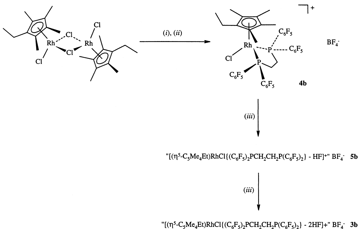
Scheme 2. (i) \text{NH}_4\text{BF}_4 , methanol; (ii) \text{dfppe} , dichloromethane; (iii) ethanol, heat.
