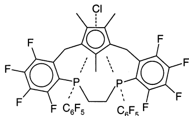
Fig. 1. Diagrammatic representation of the cation [\{\eta^5\text{-C}_5\text{Me}_3[\text{CH}_2\text{C}_6\text{F}_4\text{P}(\text{C}_6\text{F}_5)\text{CH}_2]_2\text{-1,3}\}\text{RhCl}]^+ ( 1 ) viewed along the \text{C}_5 (centroid)–Rh axis.
