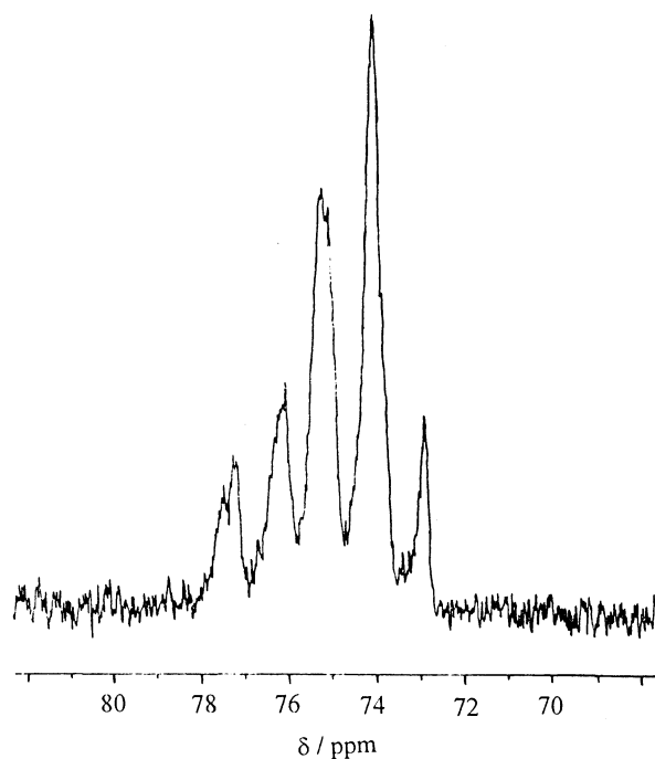
Fig. 2. ^{31}\text{P}\{^1\text{H}\} NMR spectrum of [(\eta^5\text{-C}_5\text{Me}_4\text{Et})\text{RhCl}\{(\text{C}_6\text{F}_5)_2\text{PCH}_2\text{CH}_2\text{P}(\text{C}_6\text{F}_5)_2\}-2\text{HF}]^+ \cdot \text{Cl}^- ( 3a ).
