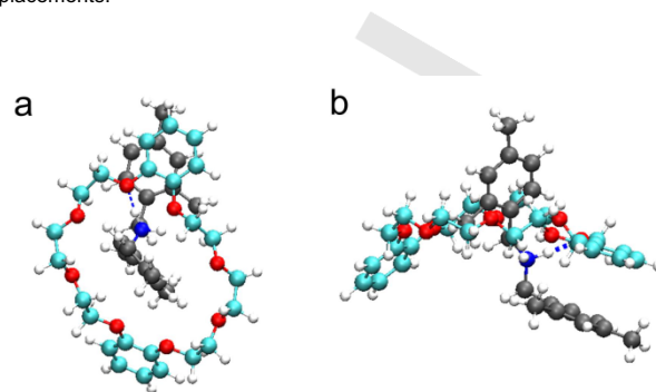
Figure 8. Vibrational modes of DB24C8 at 614 cm -1 (a) and at 809 cm -1 (b) which allow for the maximum elongation of the ring. Color codes: C = grey; O = red; H = white. The green arrows indicate the direction of the atomic displacements.
