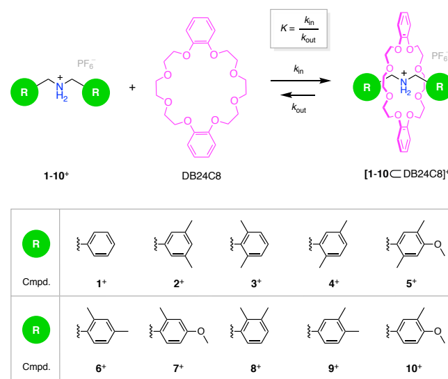
Scheme 1. Structure formulas of the investigated molecular components and their self-assembly into (pseudo)rotaxane species.
