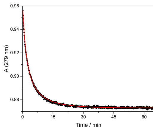
Figure 5. Time-dependent absorption changes at 279 nm recorded upon mixing DB24C8 and 4 + in CH 2 Cl 2 at 298 K. The red line represents the data fitting. Concentrations after mixing: [DB24C8] = 1.6 \times 10^{-4} M, [ 4 + ] = 1.5 \times 10^{-4} M.
