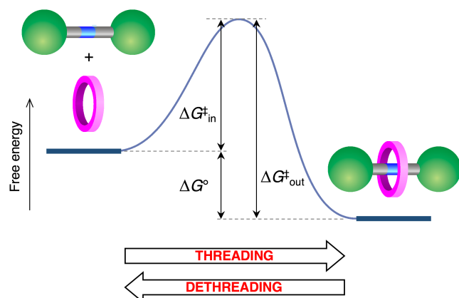
Figure 1. Schematic potential energy profile describing the threading and dethreading of molecular ring- and dumbbell-shaped components to yield (pseudo)rotaxanes.
