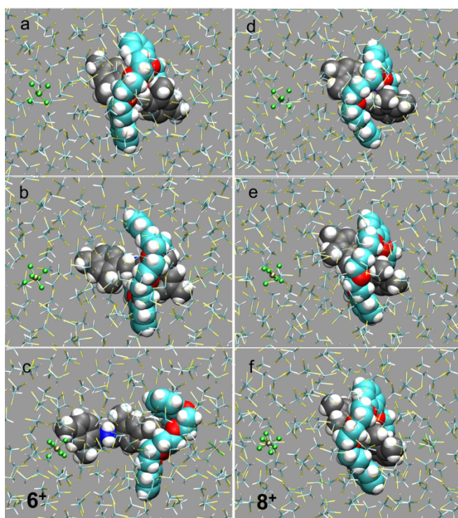
Figure 6. (a-c) Snapshots from the calculated dethreading path of the complex of DB24C8 with guest 6 + : (a) initial state (threaded); (b) transition state (partially dethreaded); (c) final state (dethreaded). (d-f) Snapshots from the metadynamics simulation of the complex of DB24C8 with guest 8 + , which predicted no dethreading. The atoms belonging to the complex are shown in a space-filling representation; color codes: C (ring) = cyan spheres; C (guest) = grey spheres; O = red; N = blue; H = white. Atoms of the solvent (CH 2 Cl 2 ) and counterion (PF 6 - ) are shown in a stick and ball-and-stick representation; respectively; color codes: C = cyan, Cl = yellow, H = white, P = dark grey, F = green.
