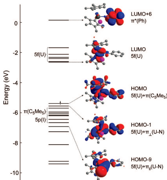
Figure 5. Occupied and virtual MO energy levels of (\text{C}_5\text{Me}_5)_2\text{U}(=\text{N}-\text{C}_6\text{H}_5)(\text{I}) ( 12 ) and plots of orbitals with significant 5f or U=N bonding character (spin-up levels are shown with unpaired electron in HOMO).
