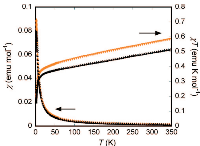
Figure 9. Magnetic susceptibilities and \chi T products of (\text{C}_5\text{Me}_5)_2\text{U}(=\text{N}-2,4,6\text{-}^t\text{Bu}_3\text{-C}_6\text{H}_2)\text{I} ( 6 , orange) and (\text{C}_5\text{Me}_5)_2\text{U}(=\text{N}-2,6\text{-}^i\text{Pr}_2\text{-C}_6\text{H}_3)\text{I} ( 10 , black) from 2 to 350 K.
