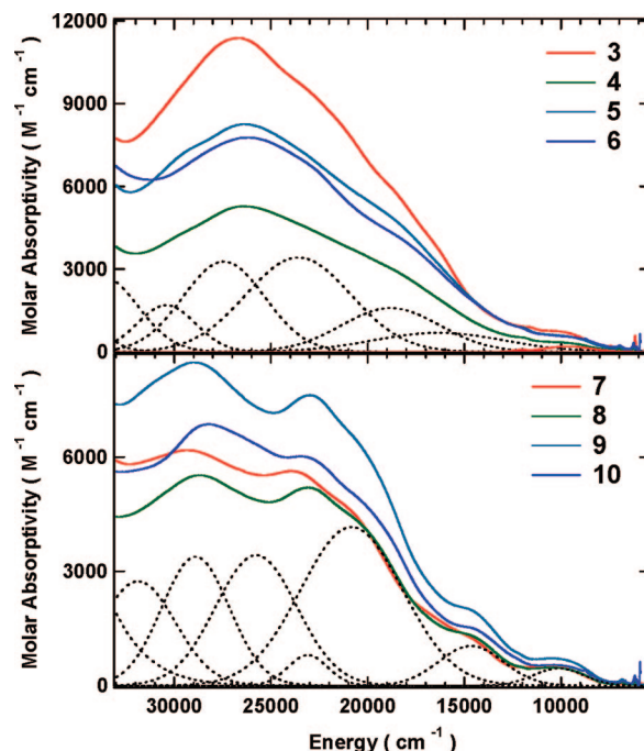
Figure 7. UV–visible–NIR absorption spectra of (\text{C}_5\text{Me}_5)_2\text{U}(=\text{N}-\text{Ar})(\text{X}) complexes 3–6 (top) and 7–10 (bottom) in toluene solution at room temperature. Dashed lines are component bands from Gaussian fit of spectra for complexes 4 and 8 .
