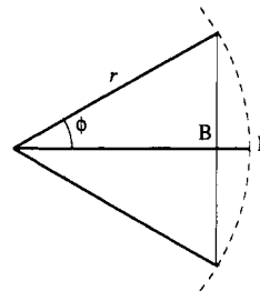
Figure 2. Displacement \overline{PB} = r - r \cos \phi \approx r\phi^2/2 caused by libration. 16-18
