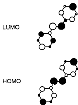
Figure 10. Relevant \pi molecular orbitals of ( E )-stilbene in the planar form with C_{2h} symmetry.
