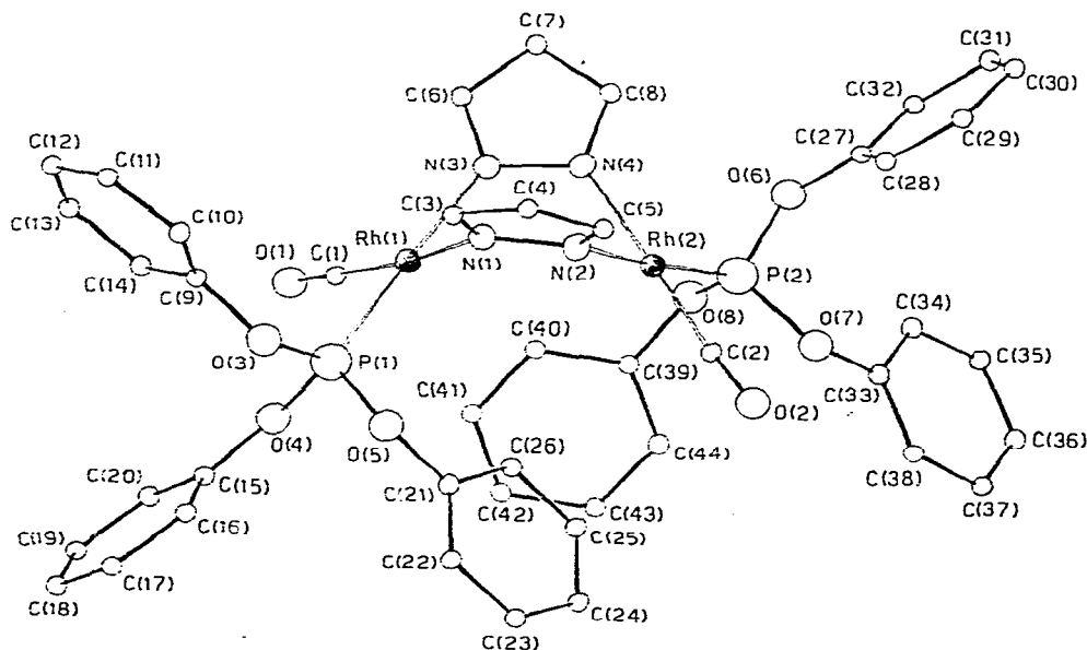
Fig. 1. View of the molecular shape of the complex [\text{Rh}(\text{Pz})(\text{CO})\text{P}(\text{OPh})_3]_2 with the atomic numbering scheme.
