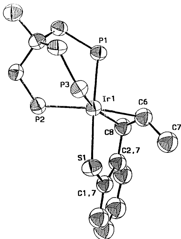
Fig. 1. ORTEP drawing of 3t ·0.5THF. All of the hydrogen atoms and phenyl rings of triphos are omitted for clarity.
