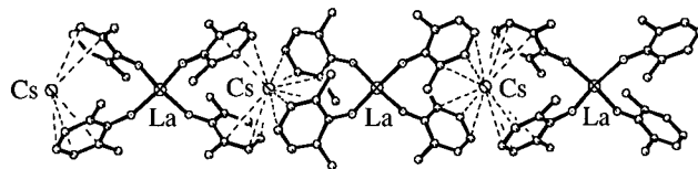
Figure 4. Ball-and-stick drawing of the extended quasi one-dimensional infinite chain structure of CsLa(OAr) 4 ( 4 ). Methyl carbon atoms of the iso -propyl groups are omitted for clarity.
