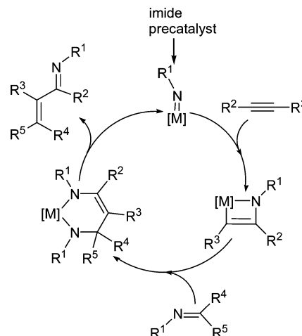
Scheme 1. Mechanism for the Catalytic Carboamination of Alkynes with Imines
