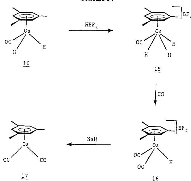
Scheme IV
