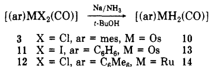
Scheme III
