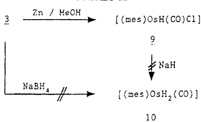
Scheme II
