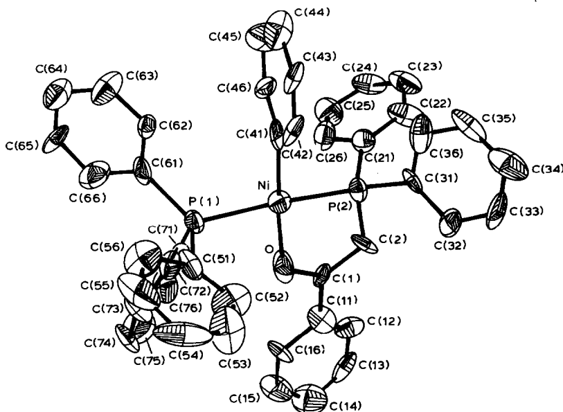
Fig. 1. Molecular structure of \text{Ph}_3\text{PNi(Ph)(Ph}_2\text{PCHCOPh)} .
