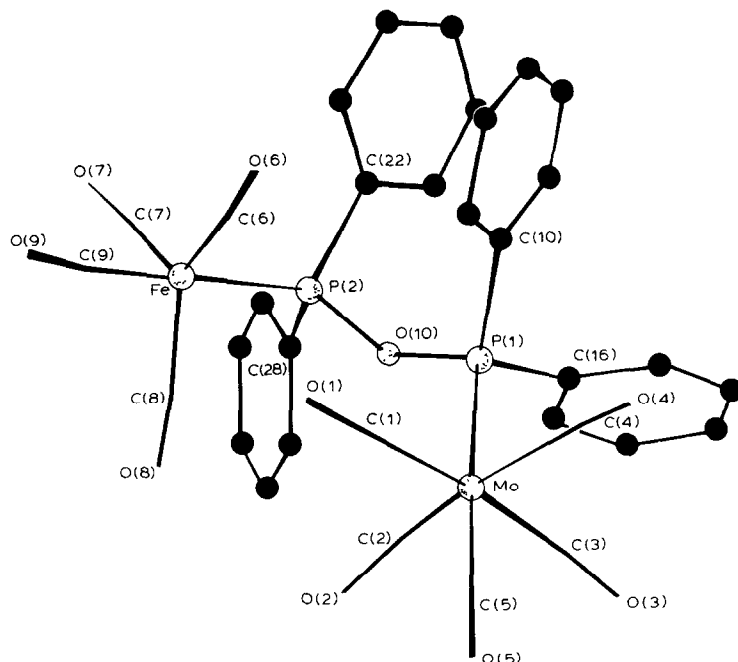
Fig. 1. The molecular structure of \text{Mo(CO)}_5\text{PPh}_2\text{OPPh}_2\text{Fe(CO)}_4 (II).
