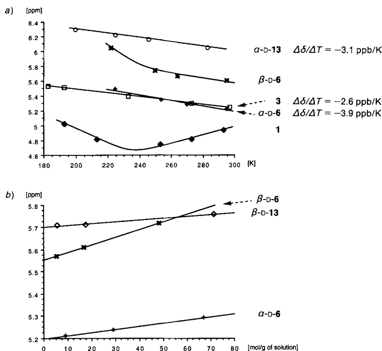
Figure. Temperature and concentration dependence of the H–N chemical shift of selected acetamides. a) Temperature dependence of the H–N chemical shifts of 1, 3, \alpha -D-6, \beta -D-6, and \alpha -D-13. b) Concentration dependence of the H–N chemical shifts of \alpha -D-6, \beta -D-6, and \beta -D-13.
