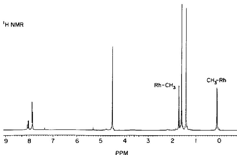
Fig. 1. 1 H NMR spectrum of (dm-pybox)Rh( cis -Me 2 )Cl (3) (in CDCl 3 ).
