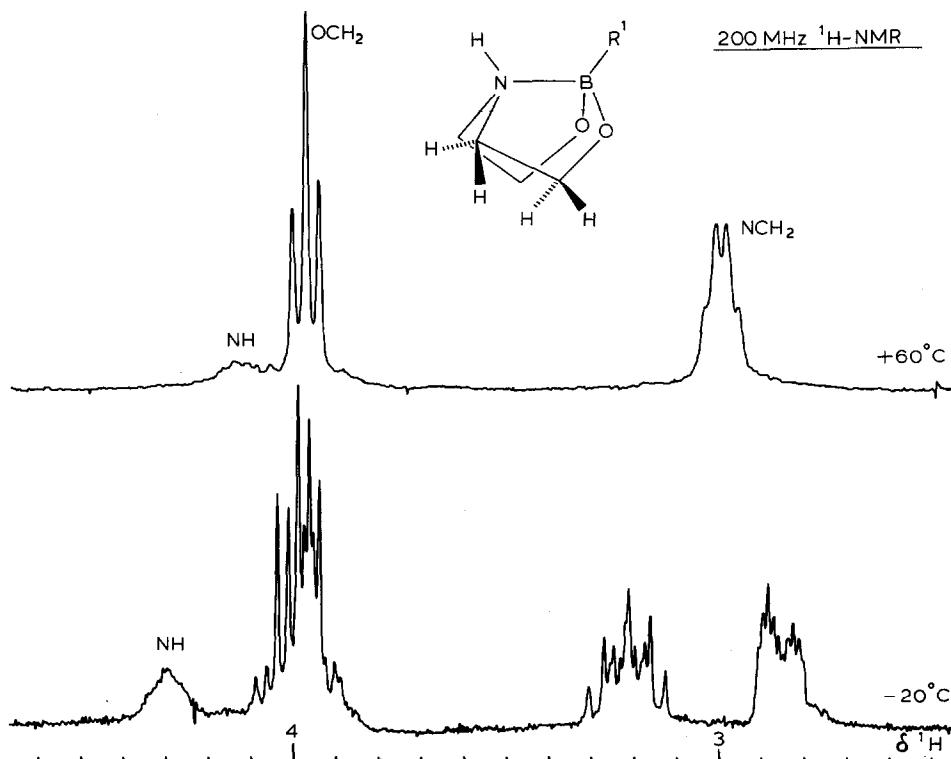
Fig. 2. 200 MHz ^1\text{H} -NMR spectra of Ia at +60^\circ\text{C} and -20^\circ\text{C} .
