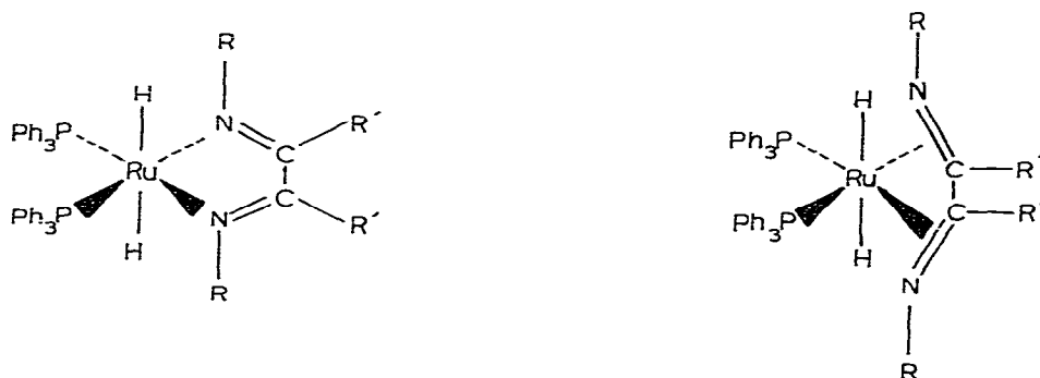
Fig. 2. Two possible structures for trans \text{RuH}_2(\text{PPh}_3)_2(\text{DAD}) .
