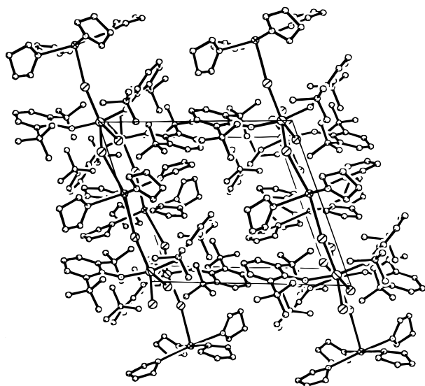
Figure 2. Packing diagram for [K(THF)_4][UCl_3(OAr)_2] ( 5 ) illustrating the infinite chain produced by the bridging potassium atoms.
