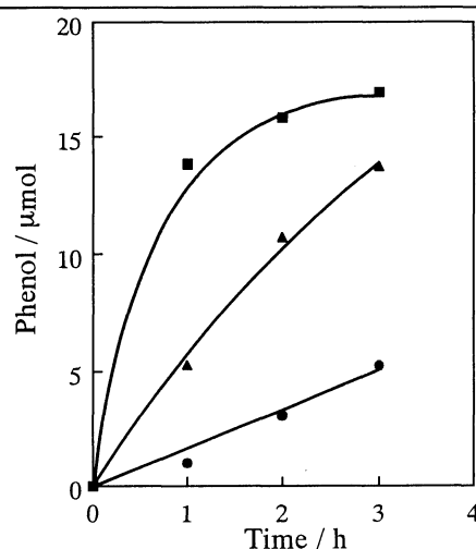
Fig. 1. Perfluorinated p -phenylenes-catalyzed photooxidation of benzene to phenol with \text{O}_2 and \text{H}_2\text{O} in acetonitrile: (●) F-OPP-3; (▲) F-OPP-4; (■) F-PPP- n .
