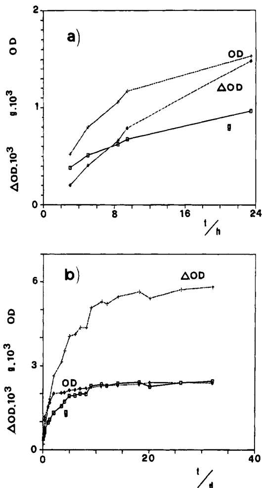
Figure 2. Variation at 675 nm of the differential optical density \Delta\text{OD} (---) the chirality factor g = \Delta\text{OD}/\text{OD} (---), and the optical density OD (···) during the formation reaction of \{\text{Cr}[(+)(S)(S)\text{Mebdtp}]_3\} in ethanol solution in 0–24 h (a) and 0–40 days (b).
