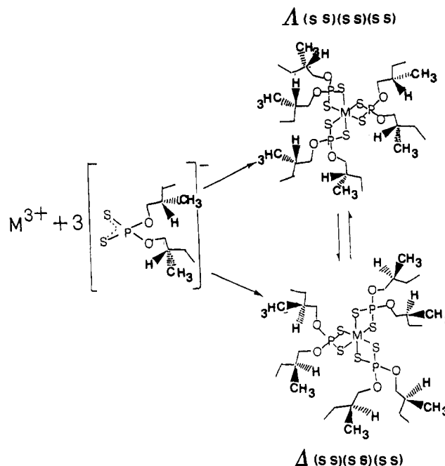
Scheme 1. Formation Reaction of Λ(−) 589 - and Δ-(+) 589 Cr[(+)(S)(S)Mebdtp] 3 and Λ ⇌ Δ Configurational Inversion in Ethanol
