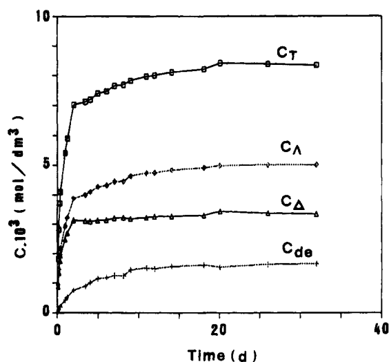
Figure 3. Variation of the concentration of complexes \{\text{Cr}[(+)(S)(S)\text{Mebdtp}]_3\} during the formation reaction: total concentration, C_T (—); concentration of the \Lambda(-)(S,S)(S,S)(S,S) diastereoisomer, C_\Lambda (···); concentration of the \Delta(-)(S,S)(S,S)(S,S) diastereoisomer, C_\Delta (---); concentration of the diastereoisomer that is in excess, C_{de} = 2C_\Lambda - C_T (-·-·-).
