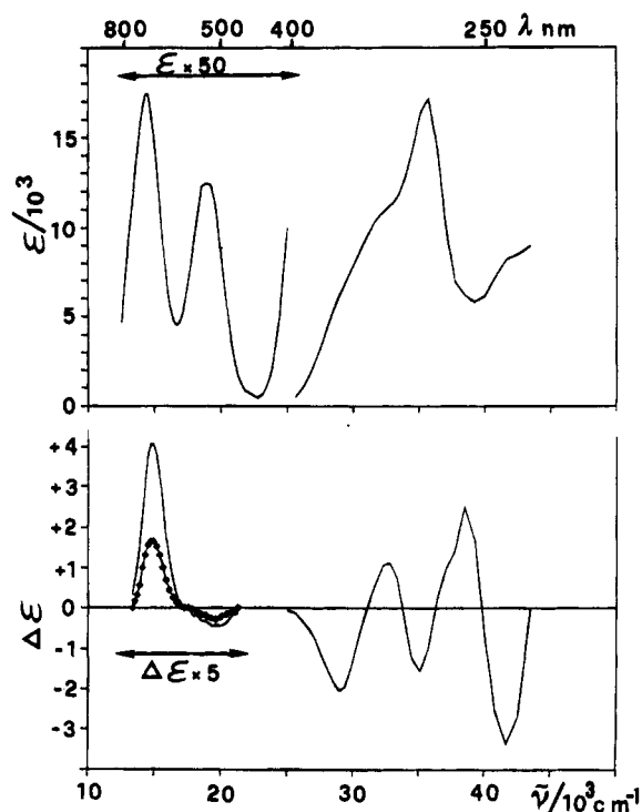
Figure 7. UV-vis and CD spectra of \{\text{Cr}[(+)\text{(S)(S)Mebdtp)}_3\} (IV) in chloroform solution 1 h after its dissolution (···) and at final equilibrium (—).
