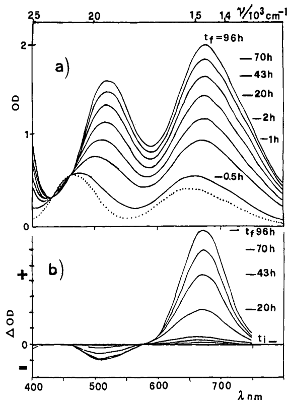
Figure 1. Formation of the \Lambda(-)\text{Cr}[(+)(S)(S)\text{Mebdtp}]_3 diastereoisomer ( t_i , starting time; t_f , final time) followed by UV-vis (a) and CD (b) in a cold ethanol reaction solution. The UV-vis spectrum of \text{CrCl}_3 \cdot 6\text{H}_2\text{O} in ethanol is shown (···).
