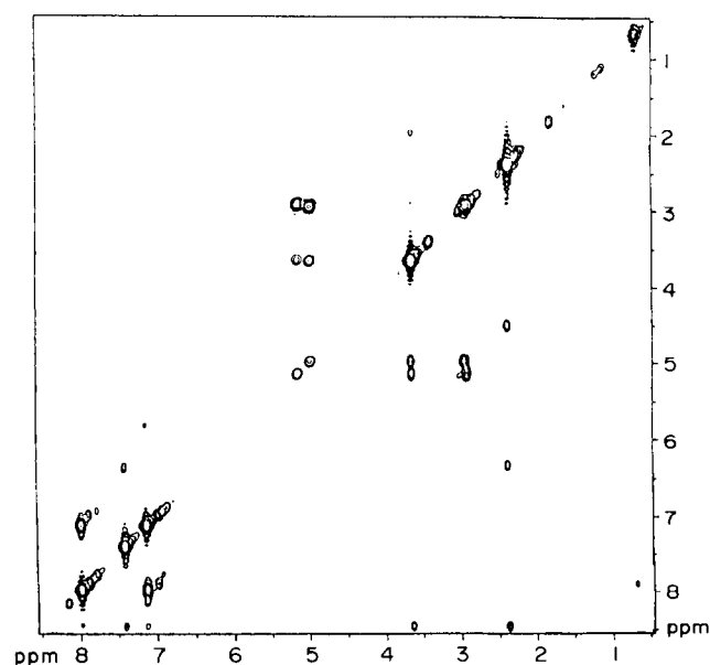
Fig. 1. COSY NMR spectrum of [Pd 2 (μ-Stol) 2 (η 3 -C 3 H 5 ) 2 ] in CDCl 3 at 500 MHz.
