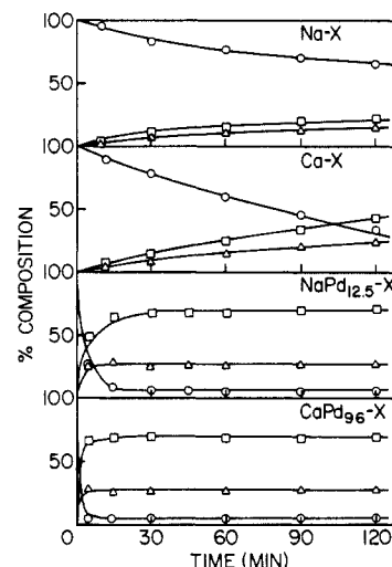
Figure 2. Isomerization of 1-butene on \text{O}_2 -pretreated zeolites. Reaction conditions: catalyst 0.05 g, P^0_{\text{C}_4\text{H}_8} = 400 Torr, reaction temperature 50 °C. Key: \circ , 1-butene; \triangle , cis-2-butene; \square , trans-2-butene.
