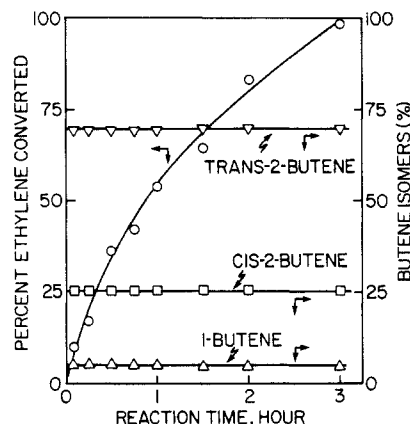
Figure 1. Ethylene dimerization on \text{O}_2 -pretreated \text{CaPd}_{9.6}\text{-X} zeolite. Reaction conditions: catalyst 0.05 g, P^0_{\text{C}_2\text{H}_4} = 400 Torr, reaction temperature 50 °C.
